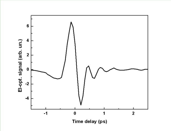
Time-domain signal
