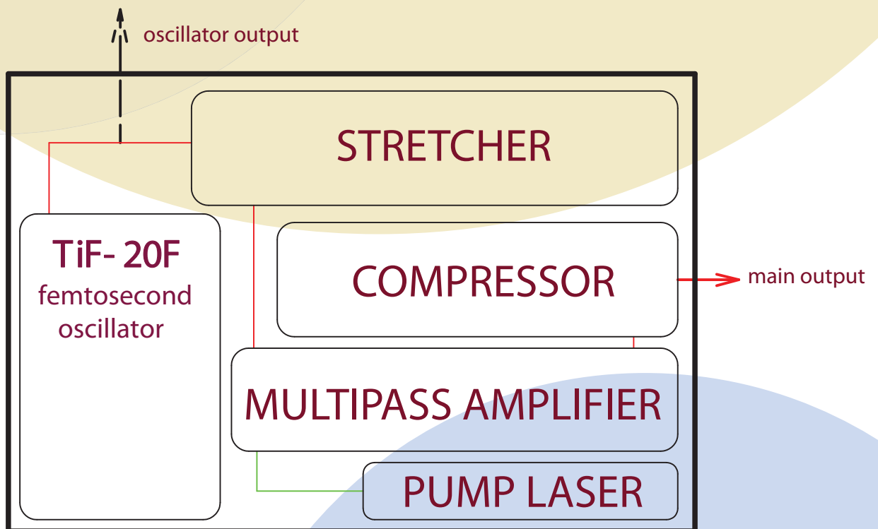
Multus MPAPOP Amplifier Layout
