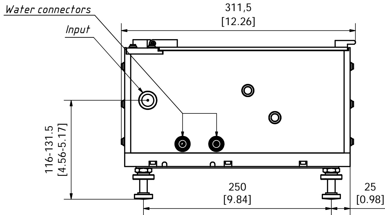
Input End View
