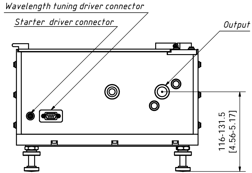
Output End View
